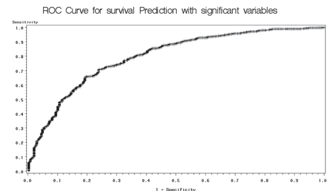
Figure 3 ROC plot for Logistic regression on survival prediction. This figure presents the ROC plot obtained when applying logistic regression for survival prediction, using only significant variables. Tables 8 and 9 contain AUC (area under curve) results for the other machine learning methods and the other prediction scenarios.
