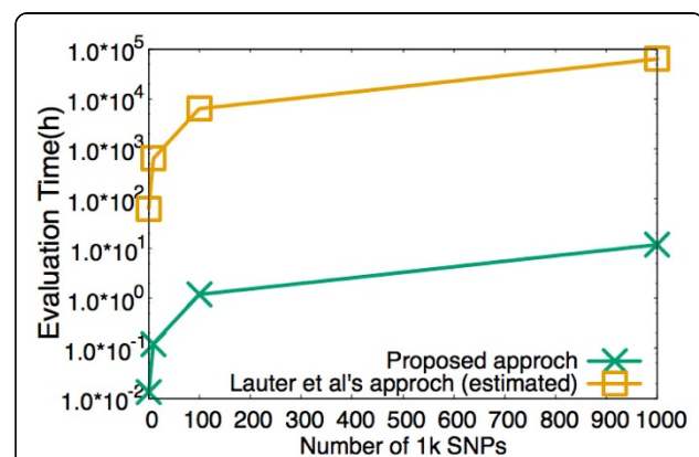
Figure 2 Benchmark for outsourcing \chi^2 test with 1.0 \times 10^4 subjects.
